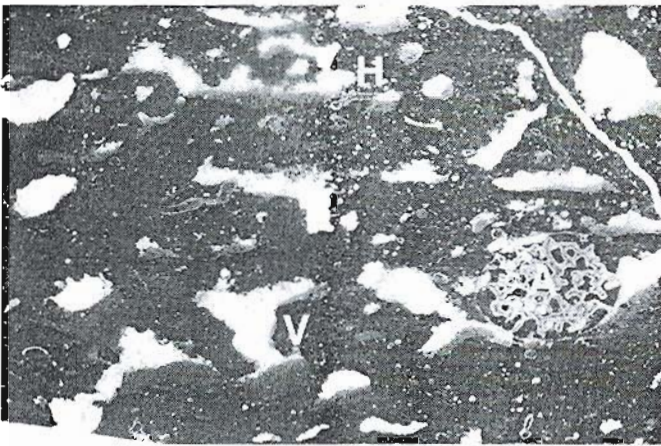
Figure 4. Microfacies 9 Peloidal and fenestral wackestone Grams of dissolved Amphipora (A) and calcispheres. Facies extremely peloidal. Both vertical (V) and horizontal (H) fenestrae displayed, each with an internal sediment-fill at base. Fenestrae 1-2mm wide. Sample number BW52, 29.8m from base of Broadridge Quarry section. Field of view 12mm x 7mm.
