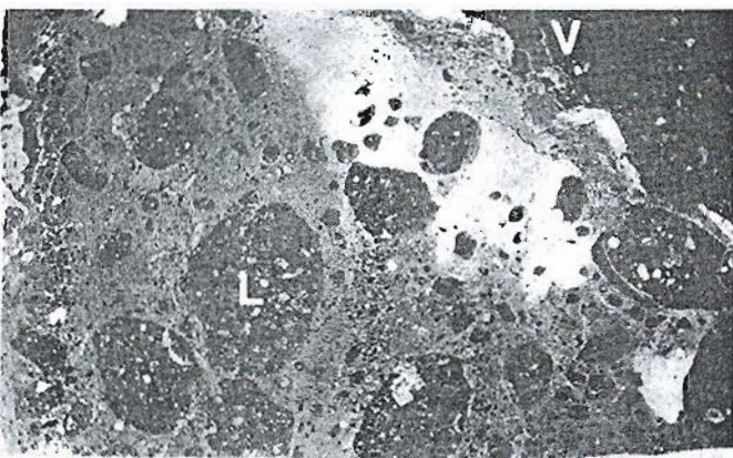
Figure 5. Microfacies 13. Immature palaeosol 2-3mm diameter, subrounded lithoclasts (L) exhibiting floating texture. Wispy sediment-filled veins (V) representing drying and cracking of sediment due to prolonged exposure. Matrix extremely mottled. Sample number BW1, 0.5m from base of Broadridge Wood Quarry section. Field of view 12mm x 7mm.
