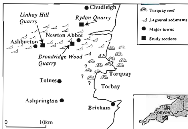
Figure 1. Location map showing non-palaeostatic distribution of facies for Lower - Middle Givetian (redrawn from Scrutton, 1977b) and distribution of quarry sections.
