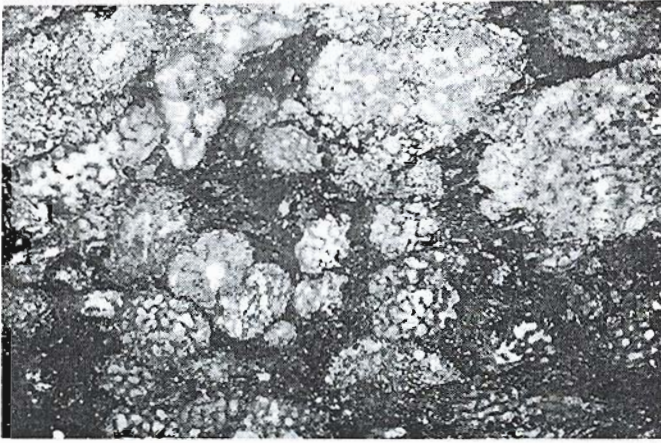
Figure 3. Microfacies 6 Amphipora floatstone Amphipora with characteristic axial canal and 3mm in diameter. Matrix composed of fine grained dolomite rhombs. Sample number BW24, 17.1m from base of Broadridge Quarry section. Field of view 12mm x 7mm.
