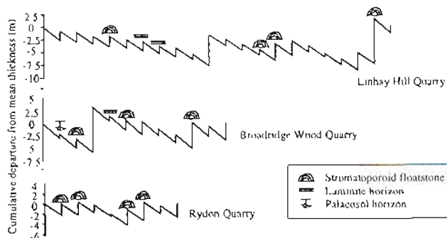
Figure 8. Fischer plots for Linhay Hill Quarry, Broadbridge Wood Quarry and Rydon Quarry. Potential correlative horizons are shown (stromatopora floatstones, laminite horizons, palaeosol horizons). Note that there appears to be little correlation between sections on the bases of cycle thickness pattern or location of distinctive beds.
