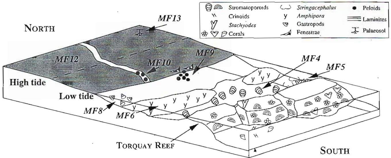
Figure 2. Palaeoenvironmental reconstruction for early - middle Givetian, showing distribution of microfacies.
